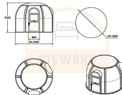
3m Clear Bubble Tent (mm)
