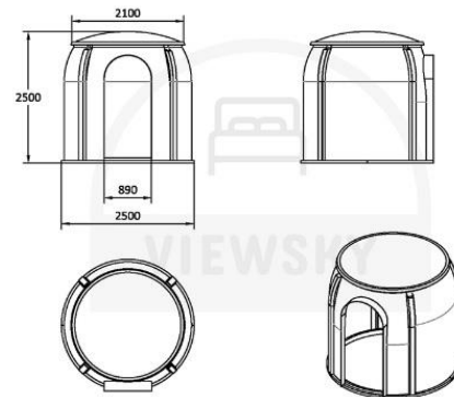
2.5m Clear Bubble Tent (mm)
