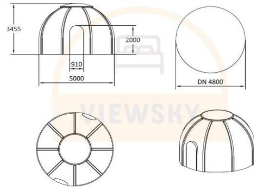
5m VIEWSKY Clear Bubble Tent (mm)
