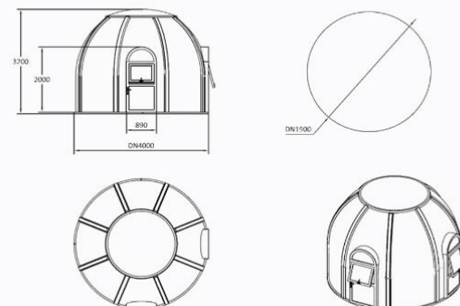
4m VIEWSKY Clear Bubble Tent (mm)
