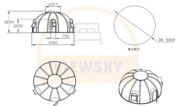
6m VIEWSKY Clear Bubble Tent (mm)
